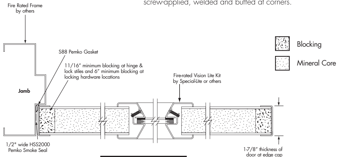
Horizontal Section
