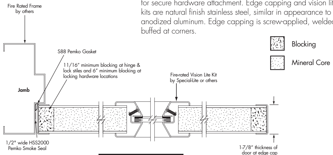
Horizontal Section
